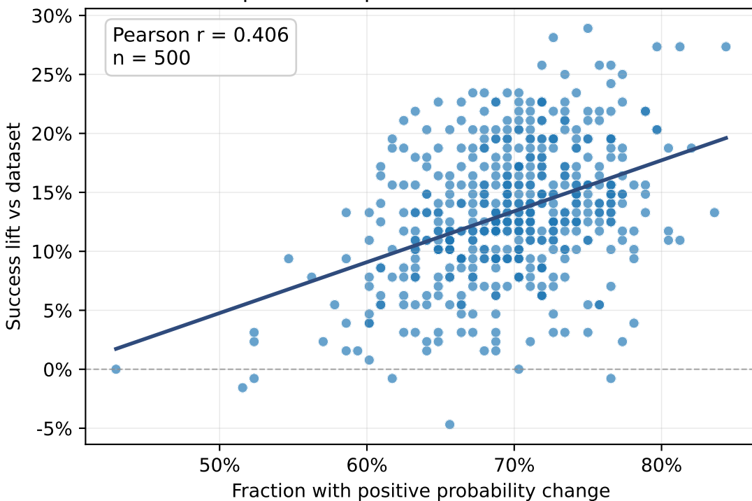
train: prob delta positive rate vs success lift
