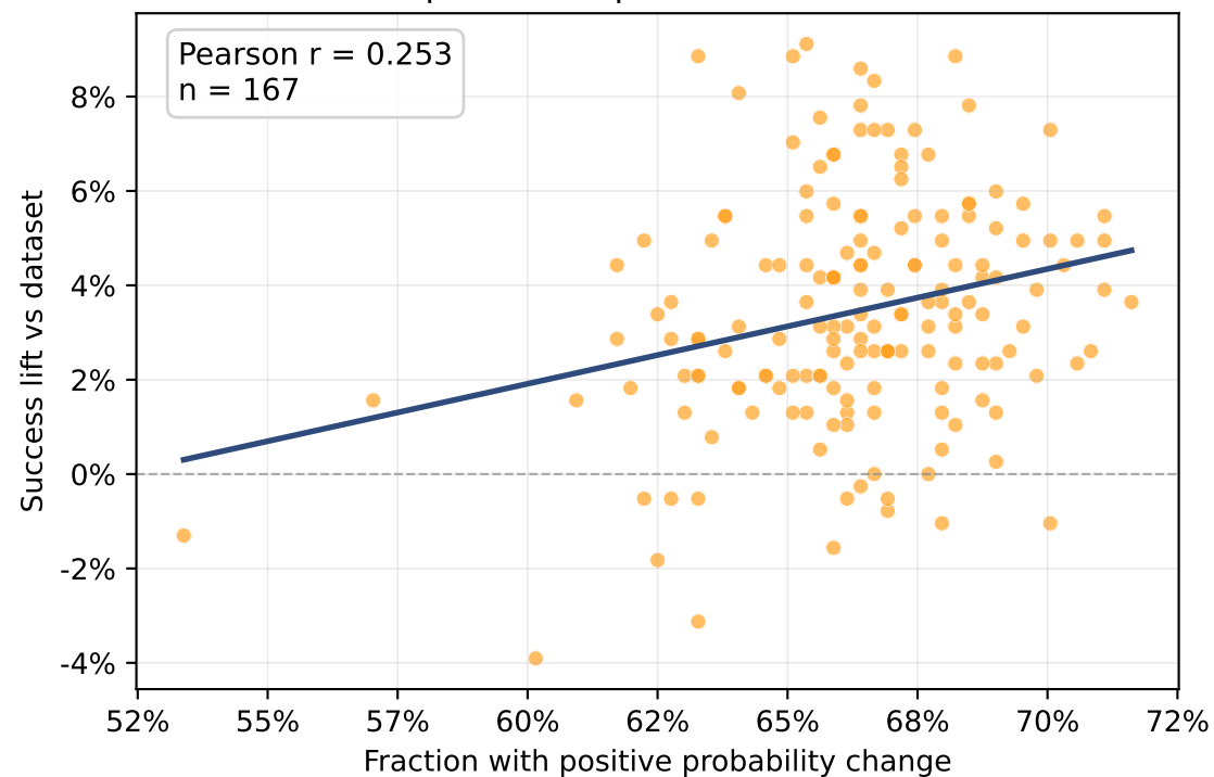
validation: prob delta positive rate vs success lift
