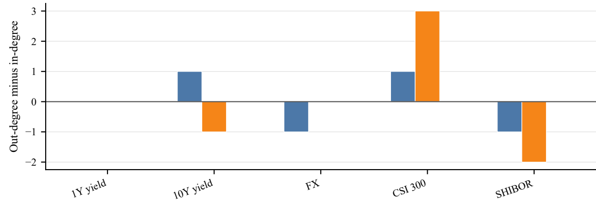
VAR-GC PCMCI-ParCorr TE Real Market Net Causal Degree
