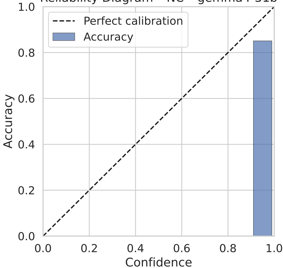
Reliability Diagram - NC - gemma4-31b
