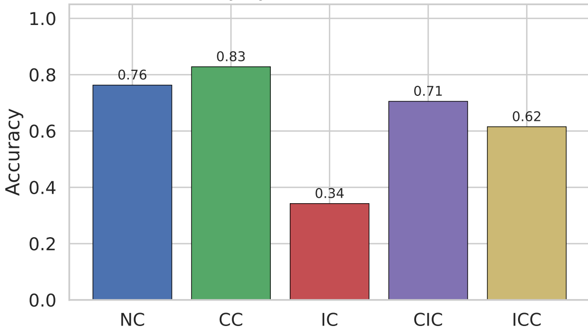
Answer Accuracy by Context Condition – llama3.1-8b
