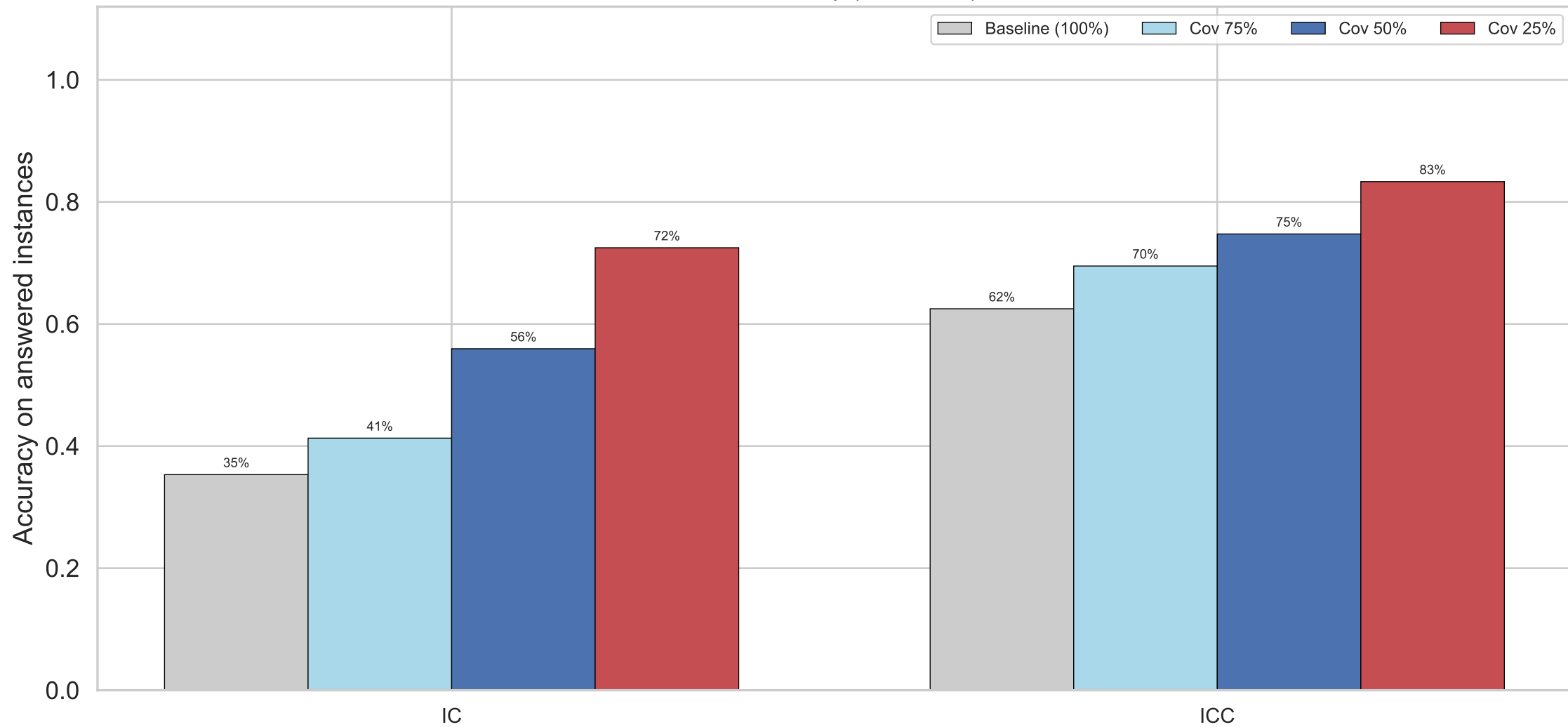
Selective Prediction Accuracy (Combined) — llama3.1-8b
