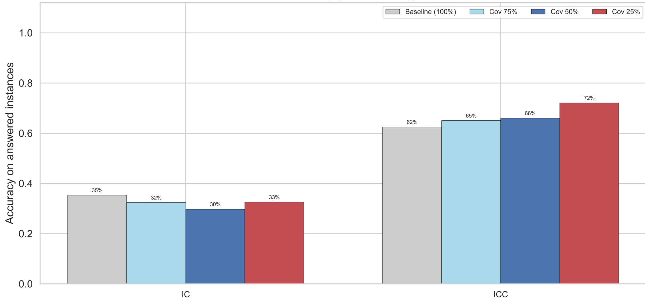
Selective Prediction Accuracy (Confidence-only) — llama3.1-8b
