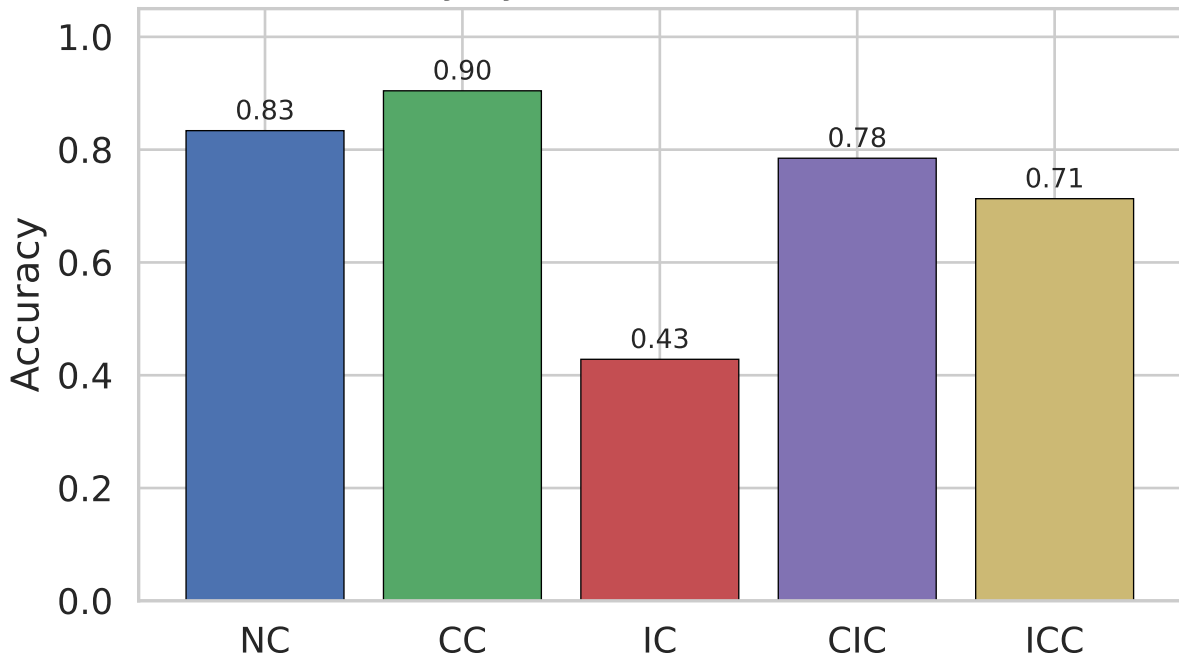
Answer Accuracy by Context Condition – meditron3-8b
