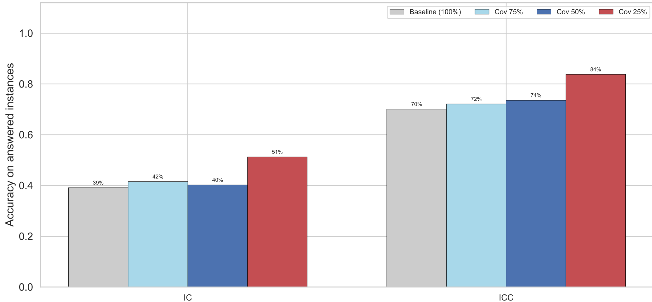
Selective Prediction Accuracy (Confidence-only) — meditron3-8b
