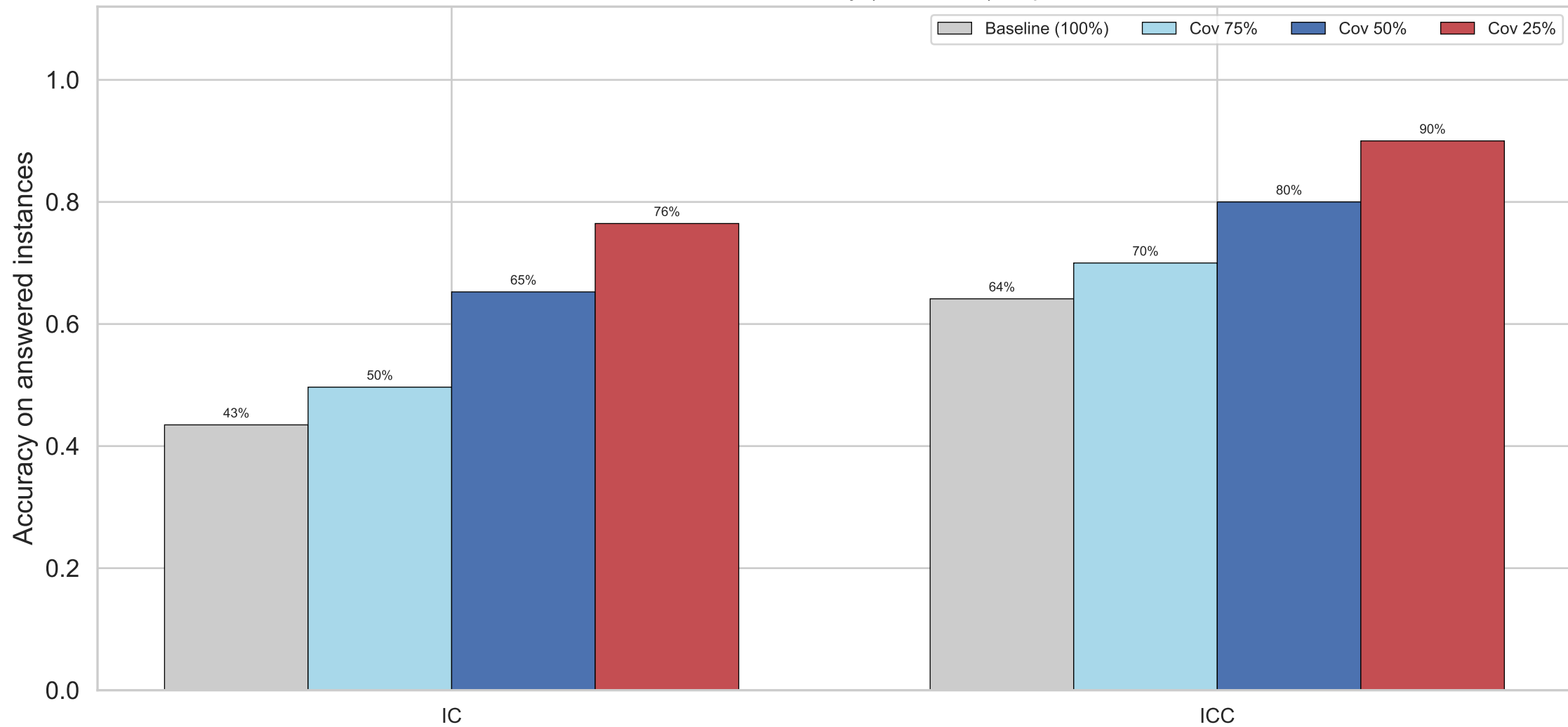
Selective Prediction Accuracy (Combined) — phi4-14b
