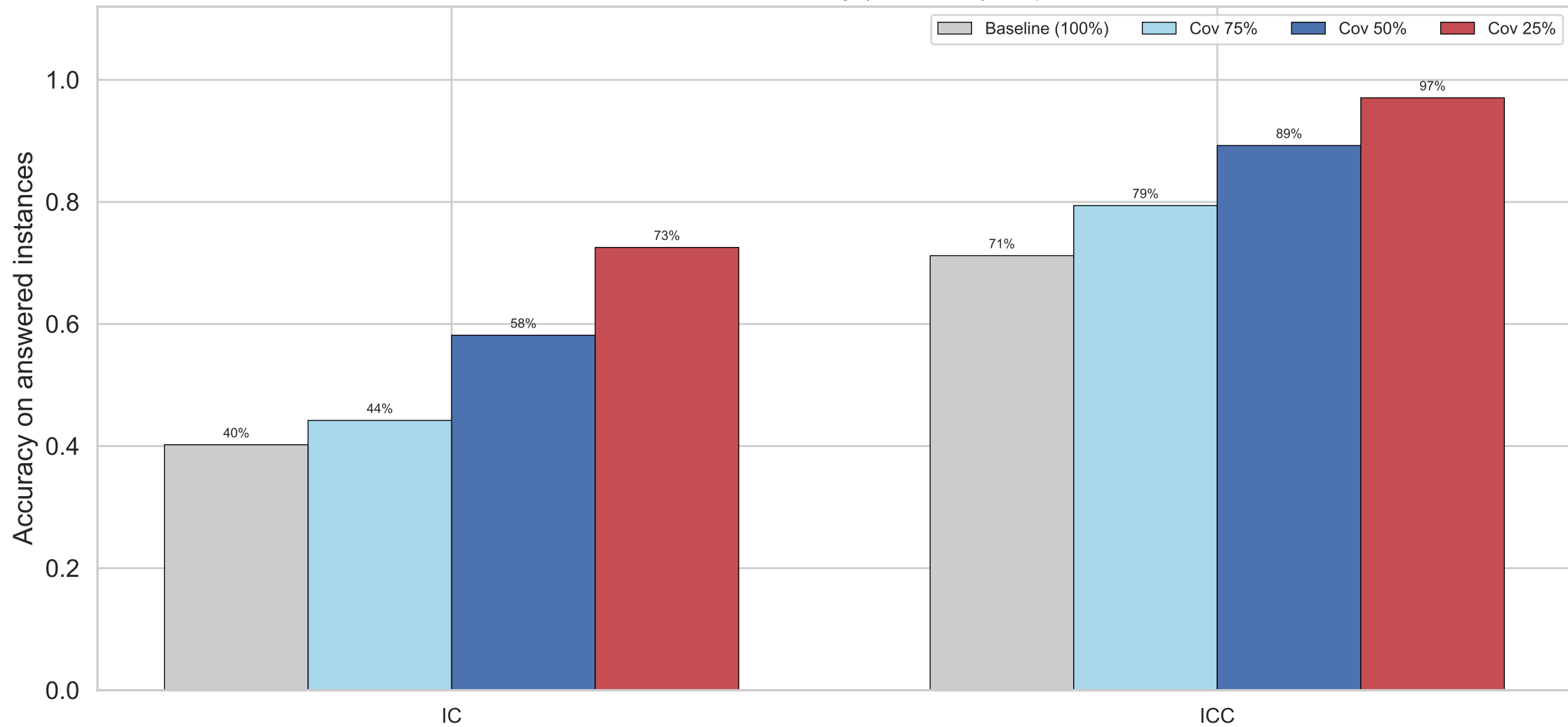
Selective Prediction Accuracy (Combined) — qwen3-4b
