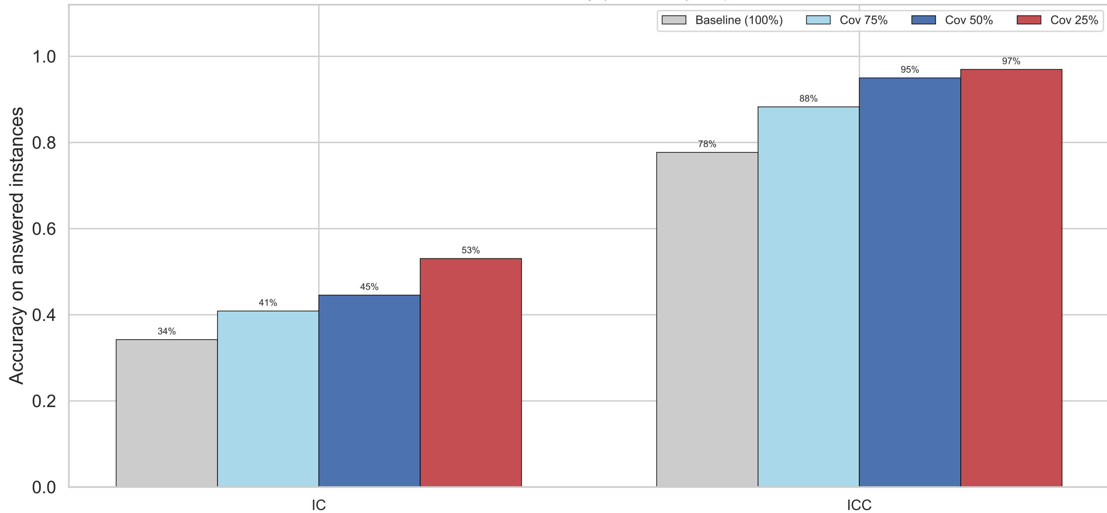
Selective Prediction Accuracy (Combined) — qwen3.5-9b
