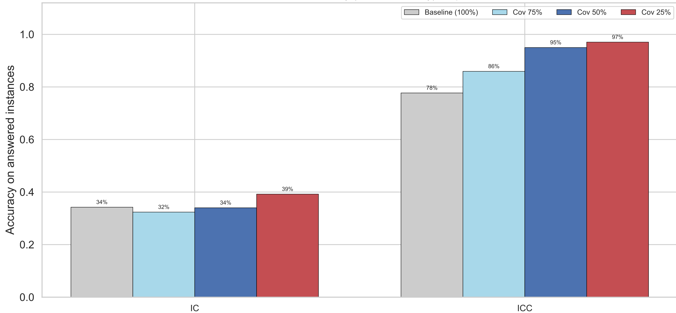
Selective Prediction Accuracy (Confidence-only) — qwen3.5-9b
