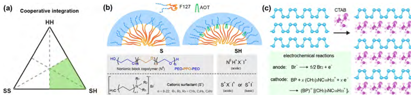
Figure 8. Interaction framework—cooperative integration can be verified with existing examples. (a) The cooperative integration diagram. (b) Synthesis of mesostructured inorganic materials often involves self-assembly of inorganic precursors (positively charged I^+ or negatively charged I^- ) with cationic surfactants ( S^+ ) or nonionic block copolymers ( N^0 ). The soft–hard (SH) interactions can involve protonation ( H^+ ) and anion coupling ( X^- ), and occur in either acidic or basic conditions. In block copolymer-based synthesis, e.g., with pluronic F127, the hydrophilic segments such as PEO are inserted inside the inorganic walls, producing a graded regime. The addition of cosurfactant such as sodium bis(2-ethylhexyl) sulfosuccinate (AOT) can tune the interface chemistry and the curvature. (c) Electrochemical intercalation of black phosphorus (BP) by CTAB molecules produces a soft–hard superlattice structure. Electrochemical reactions are shown in the lower left panel. As the superstructure cannot be formed by either the black phosphorus or the CTAB molecules alone, the cooperativity at the soft–hard interfaces is the key to the final composite structure.
