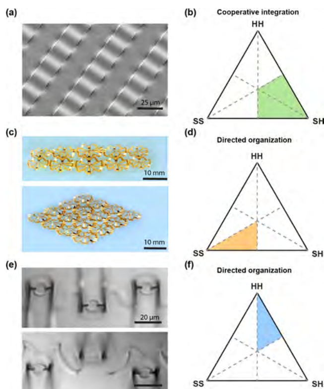
Figure 13. Interaction between soft substrates and hard electronics produces stretchable and three-dimensional devices. (a) Interaction between the stretchable substrate and silicon material allows the formation of highly uniform ribbons. Reproduced with permission from ref 200. Copyright 2006 AAAS. (b) Cooperative integration, SH > SS , SH > HH . The wavy structure was formed through a biphasic cooperative process. This structure cannot form with PDMS or Si nanoribbon alone. (c) Arrays of three-dimensional multifunctional mesoscale frameworks for holding and recording electrical activity in spheroid organoids. Reproduced with permission from ref 211. Copyright 2021 AAAS. (d) Directed organization, SS > SH > HH . The local bonding sites and the elastomer substrate enable 2D–3D transformation. (e) Stress between the hard (metal) and soft (SU-8) materials allows for transistor positioning in a recording device. Reproduced with permission from ref 212. Copyright 2012 Springer Nature. (f) Directed organization, HH > SH > SS . The residual stress from multiple material layers enables the 2D–3D transformations.
