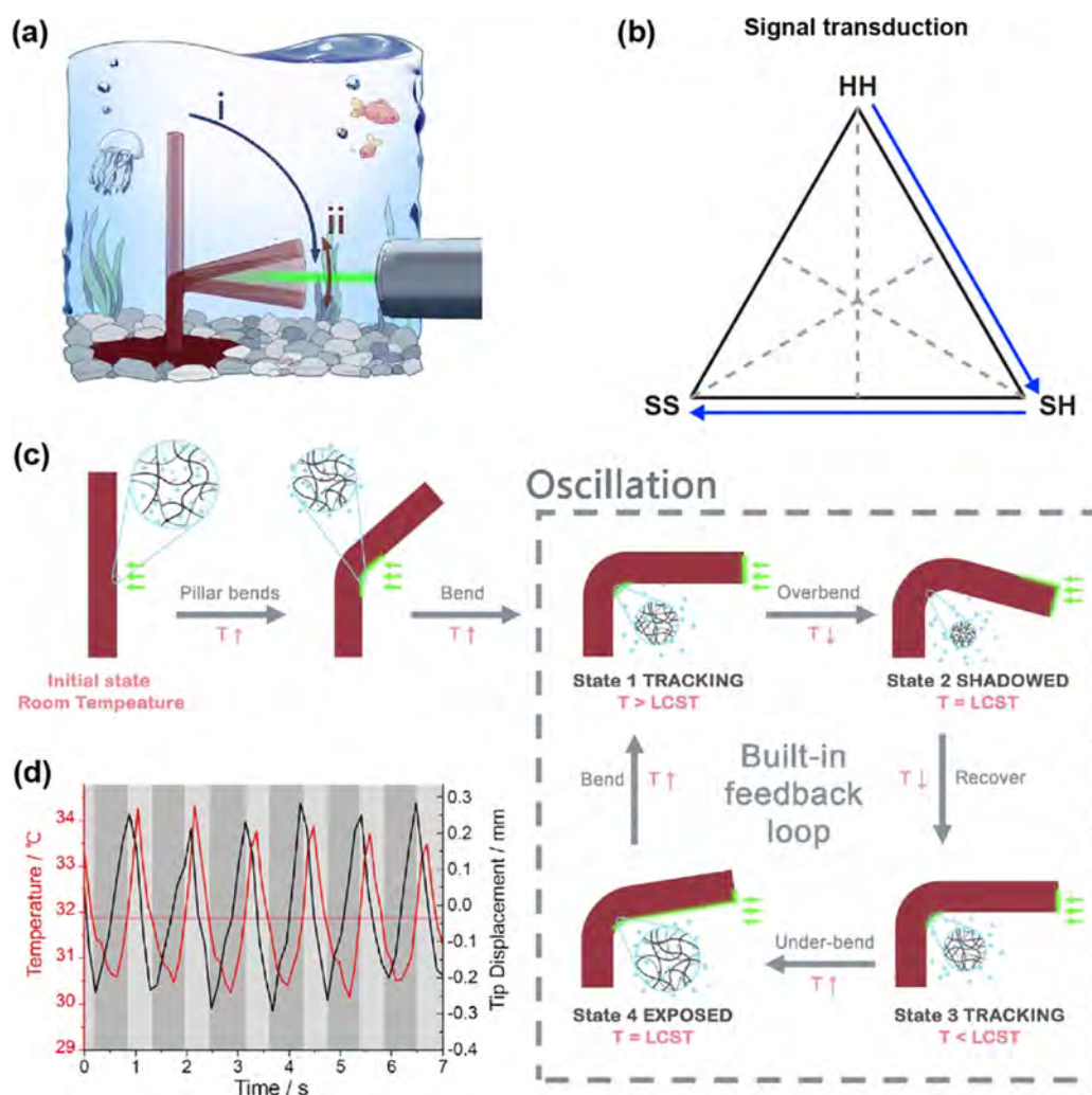
Figure 22. Phototactic gels allow the creation of oscillators that can be used for light-driven motion. (a) Schematic of the laser-driven oscillating pillar made of the phototactic gel. (b) Soft–hard interaction framework. The signal transduction follows HH > SH > SS . (c) Mechanism of oscillating motion. Self-shadowing of the pillar's inner surface creates out-of-equilibrium condition and negative loop driving the reciprocal motion. (d) Tip displacement and local temperature in the hinge during motion. The 90^\circ shift between the curves is in agreement with the proposed motion mechanism. Reproduced with permission from ref 230. Copyright 2019 AAAS.
