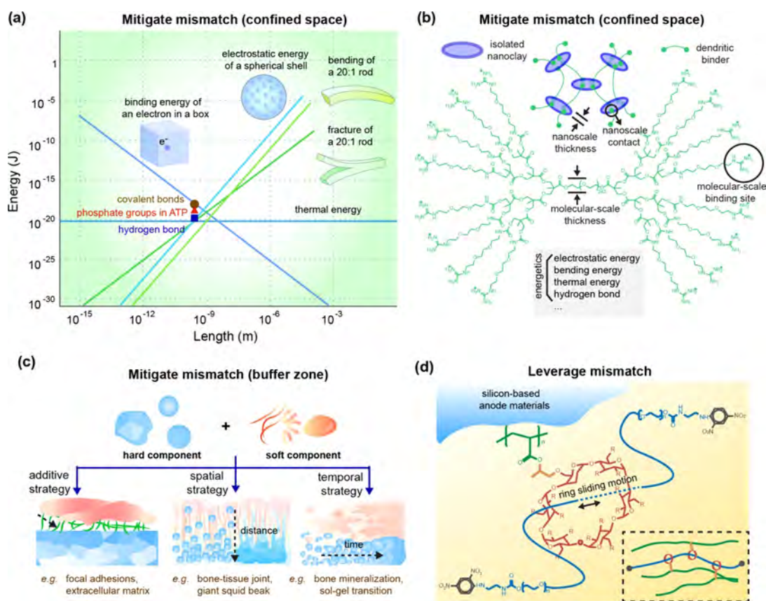
Figure 4. Processes at soft–hard interfaces are unique. (a) Although different energies display different dependence on object size or dimensions, they converge at the molecular and nanoscopic scale. At this length scale, efficient signal transduction and minimal mismatches are expected at soft–hard interfaces. At this size regime, the boundaries between soft and hard materials, and the boundaries between living and nonliving systems, become blurred. This energy convergence can explain the critical roles of nanoscale interfacial processes at many soft–hard interfaces. 36 Reproduced with permission from ref 96. Copyright 2019 Nature Springer. (b) Dendritic binders and nanoclays self-assemble to form stable hydrogel. The feature sizes of the building blocks are at the molecular and nanoscopic levels, where multiple energy terms show similar amplitude such that the soft–hard interfaces can establish in a seamless manner. (c) To mitigate interfacial mismatches, additional buffer mechanisms are available. These mechanisms include the use of connecting linkers and deposits (additive strategy), the formation of a modulus gradient over the distance between the soft and hard phases (spatial strategy), and gradual and less perturbative condensation of the hard component at the interface (temporal strategy). (d) The soft–hard interfaces can produce the strain hotspots, which may be leveraged for special chemical processes or applications. For example, ring sliding of polyrotaxane close to the silicon/binder interfaces can be triggered during the operation of silicon-based battery anode.
