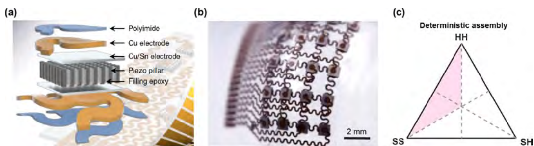
Figure 15. Flexible ultrasonic device has high mechanical resilience and can conform to the skin enabling remote sensing of blood pressure. (a) Schematic of the ultrasonic device with the array of piezoelectric rods embedded in an epoxy matrix. (b) Optical image of the device under strain showing its high conformability. (c) The device was made by the deterministic assembly, where the properties of the soft and hard phases are well-defined. Reproduced with permission from ref 256. Copyright 2018 Springer Nature.
