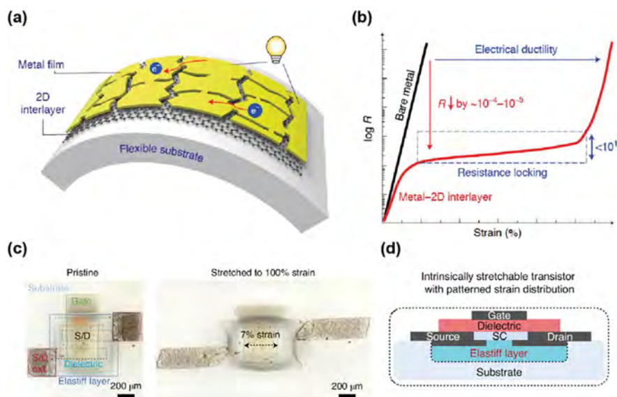
Figure 14. Atomically thin-material interlayers enable strain-resilient electrodes. (a) Schematic of a fractured metal film on single-layer graphene forming the conductive and flexible electrode. (b) Conceptual plot comparing resistance in bare metal and metal-interlayer material in the function of applied strain. The metal-interlayer material possesses a large, stable “resistance locking” region. (c) Optical image of a flexible transistor array under 0% (left) and 100% (right) deformation. The varying concentration of cross-linkers in conductive polymers allows for the fabrication of the device with the prescribed stiffness allowing redistribution of strain to the nonactive areas. (d) Representative structure of a flexible transistor device. (SC, semiconductor material) Panels a and b were reproduced with permission from ref 245. Copyright 2021 Springer Nature. Panels c and d reproduced with permission from ref 218. Copyright 2021 Springer Nature.
