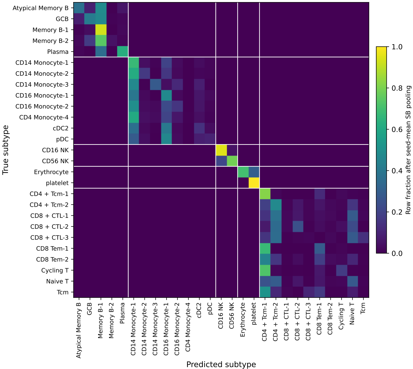
Full-budget APT MLP: true-lineage oracle
