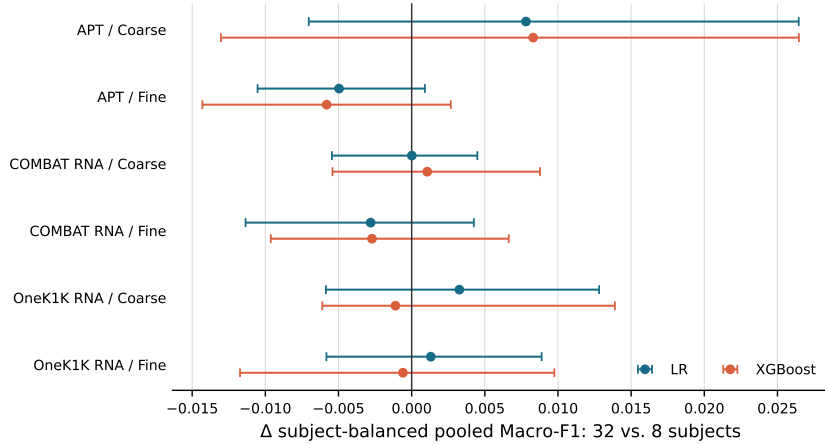
Figure 1: Class-matched fixed-total scaling across three cohorts. Each comparison freezes observed classes and exact per-class quotas before reallocating T = 6,400 training cells from 8 to 32 subjects. Points are changes in subject-balanced pooled OOF macro-F1; 95% joint intervals resample both the training-subset seed and paired held-out subjects. All 12 intervals include zero.
