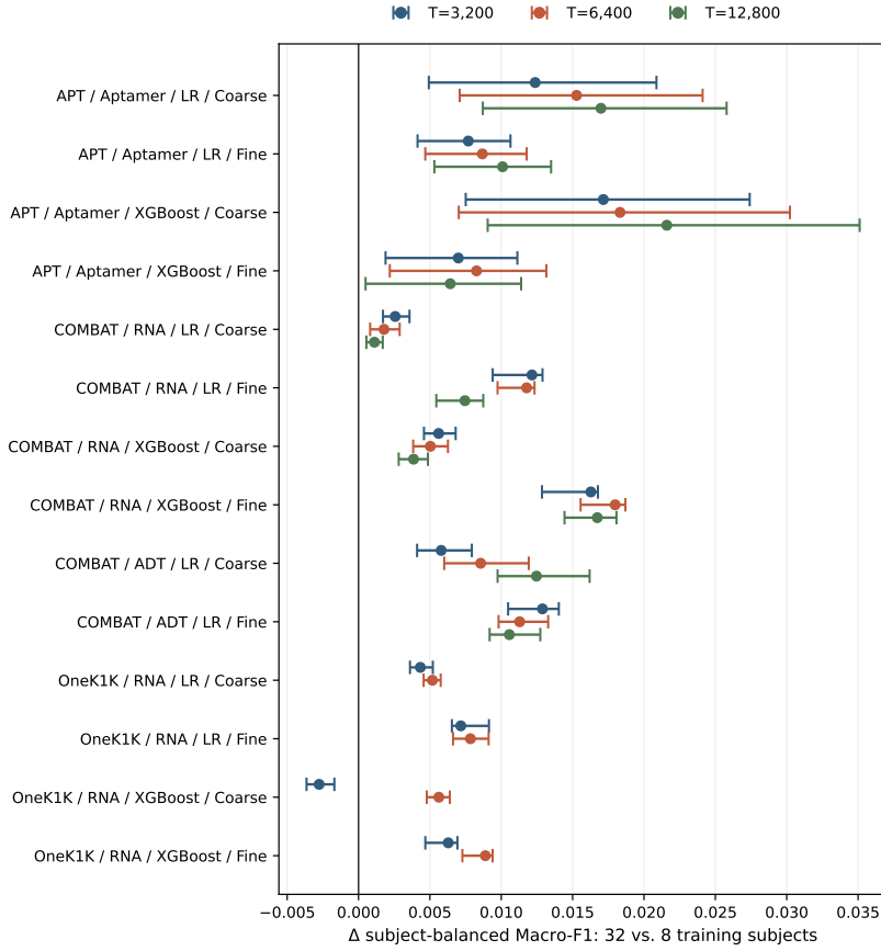
Figure 1: Cross-cohort fixed-total scaling. Points are changes in subject-balanced, subject-disjoint OOF macro-F1 when a fixed total of T training cells is reallocated from 8 to 32 independent subjects; positive values favor broader subject coverage. Bars are 95% paired subject-bootstrap intervals over fixed outer-test subjects after averaging seeds. APT, COMBAT RNA, and OneK1K RNA use LR/XGBoost; COMBAT ADT is an LR-only sensitivity. OneK1K supports two totals under its 800-cell donor threshold.
