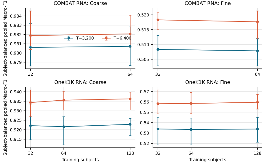
Figure 5: Class-matched LR frontier beyond 32 training subjects. Points are mean subject-balanced pooled OOF macro-F1 over 10 matched training-subset seeds; bars are empirical 95% seed intervals and therefore visualize subset sensitivity, not uncertainty of the mean. The paired joint stability intervals are reported in Table 21.
