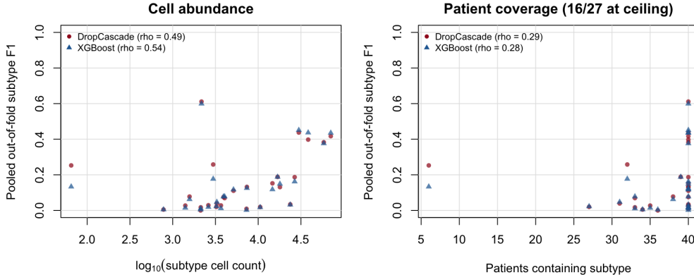
Figure 2: Per-subtype pooled out-of-fold F1 versus cell abundance (left) and patient coverage (right). Each marker is one of 27 subtypes; both models use the same ground-truth support values. Spearman correlations are marginal, and 16 of 27 subtypes occur in all 40 patients.
