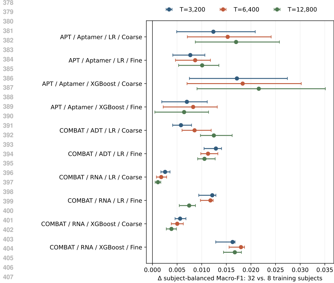
Figure 1: Cross-cohort fixed-total scaling. Points are changes in subject-balanced, subject-disjoint OOF macro-F1 when a fixed total of T training cells is reallocated from 8 to 32 independent subjects; positive values favor broader subject coverage. Bars are 95% paired subject-bootstrap intervals over fixed outer-test subjects after averaging seed-level sufficient statistics. APT uses LR and XGBoost; COMBAT RNA replicates both models, and COMBAT ADT is an LR-only modality sensitivity on the same donors and cells.
