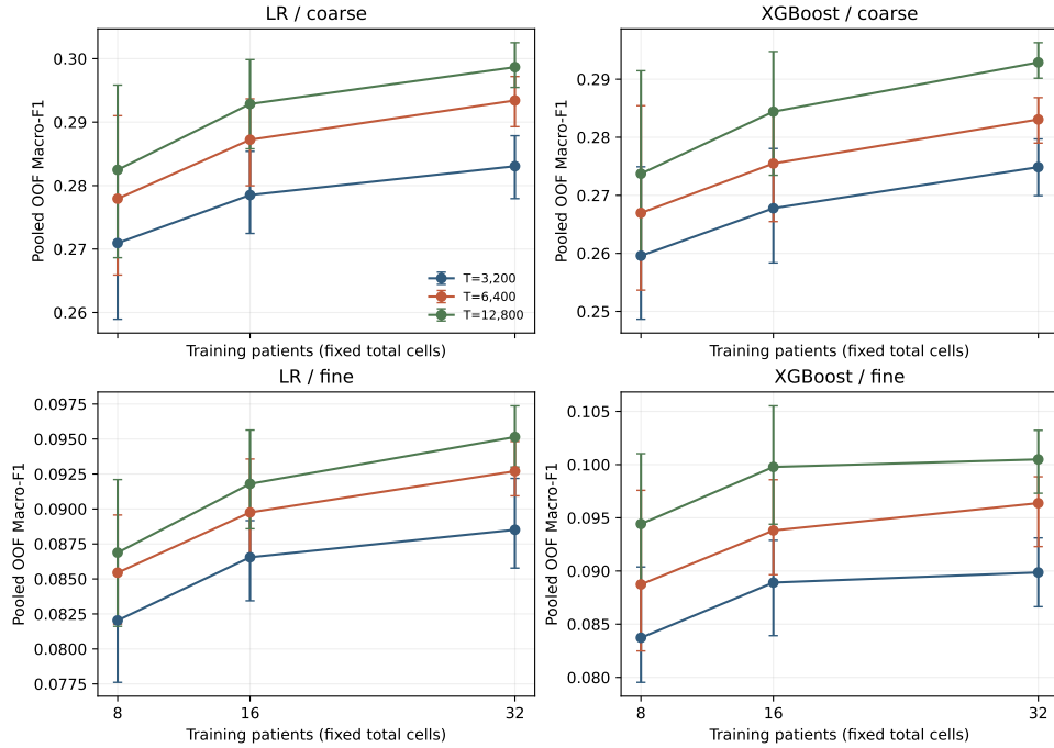
Figure 3: APT-only fixed-total response curves underlying the cross-cohort effect summary in Figure 1. Points are pooled OOF macro-F1 means over 20 matched subset seeds; bars are empirical 95% seed intervals. Patient-balanced and patient-bootstrap results are provided in the machine-readable artifacts.
