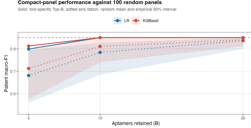
Figure 6: Patient-level disease-association macro-F1 under feature-budget controls. Solid lines show pooled out-of-fold performance obtained using fold-specific Top- B panels; dotted lines and ribbons show the mean and empirical 95% interval over 100 random-panel repeats. Each repeat shares one panel across outer folds, with models refit foldwise. The dashed line is the full 293-aptamer reference; scores pool the 40 outer-test patients once each. Because acquisition effects are unrecorded, the curves quantify redundancy of the mixed within-cohort signal rather than reduced-assay validity.
