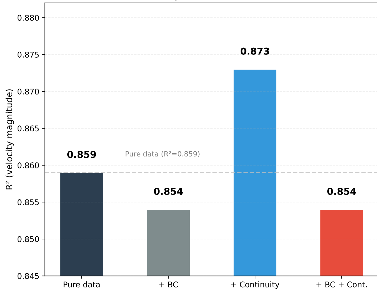
(a) Physics term ablation
