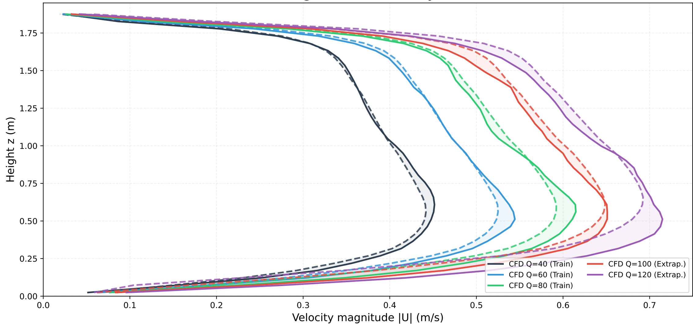
Center-blowing centerline velocity: CFD vs PINN
