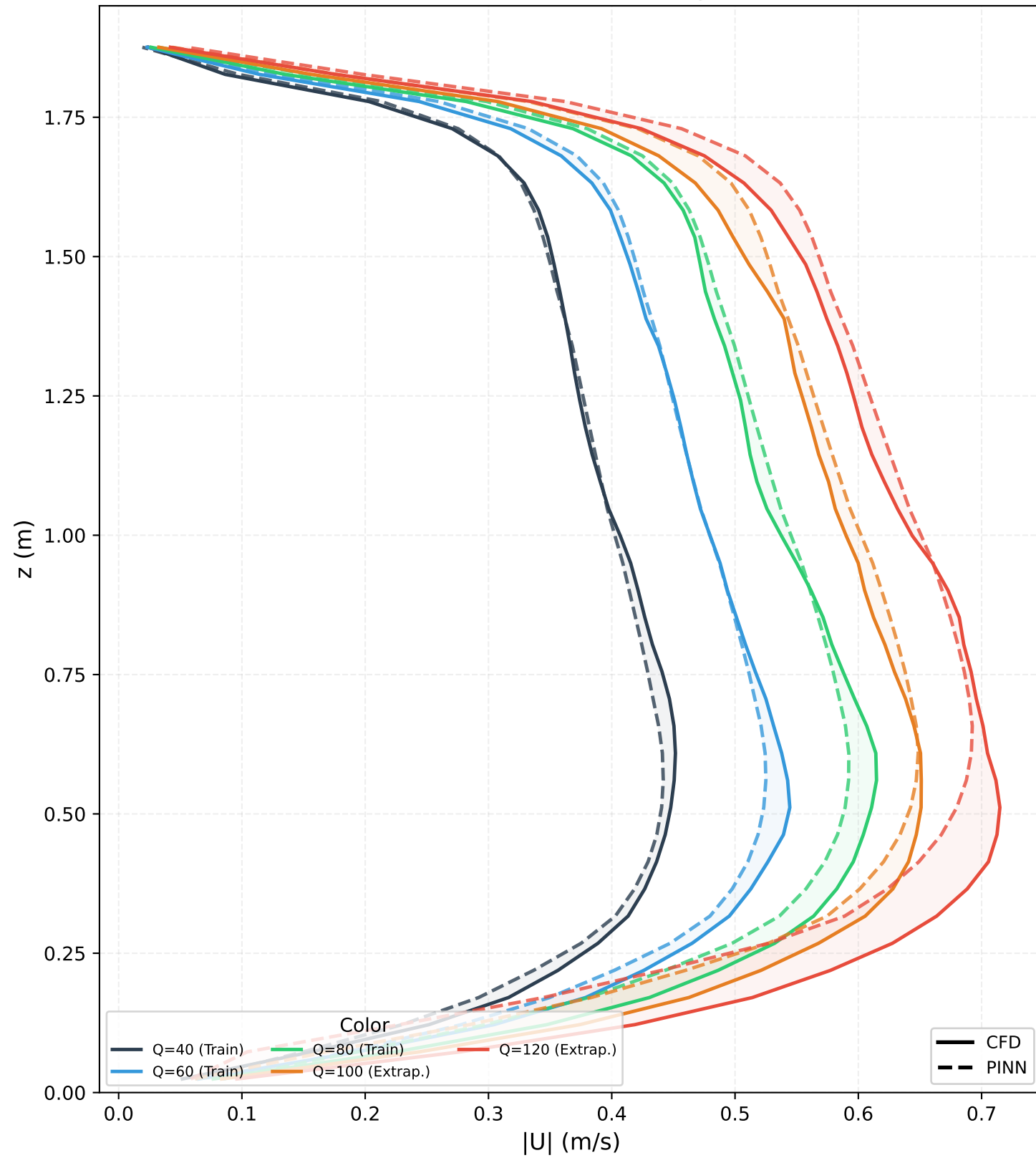
(a) Center blowing
