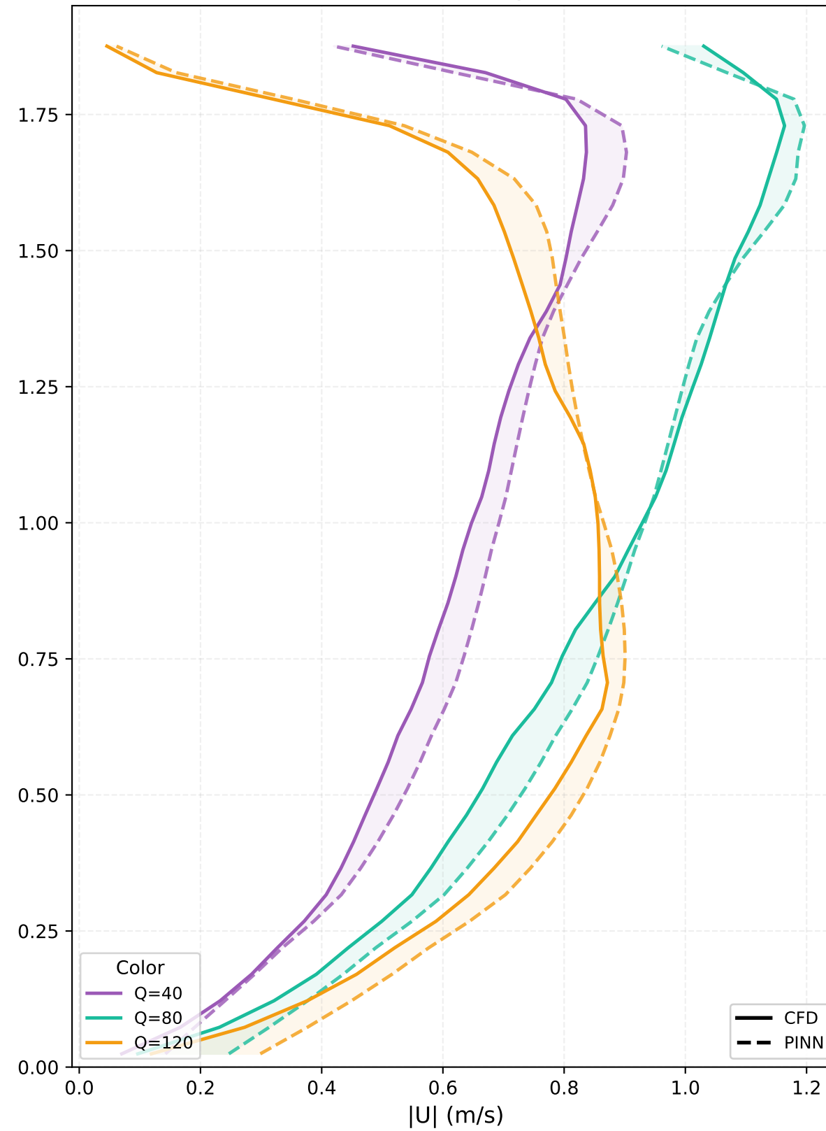
(b) Eccentric blowing (x=0.47m)
