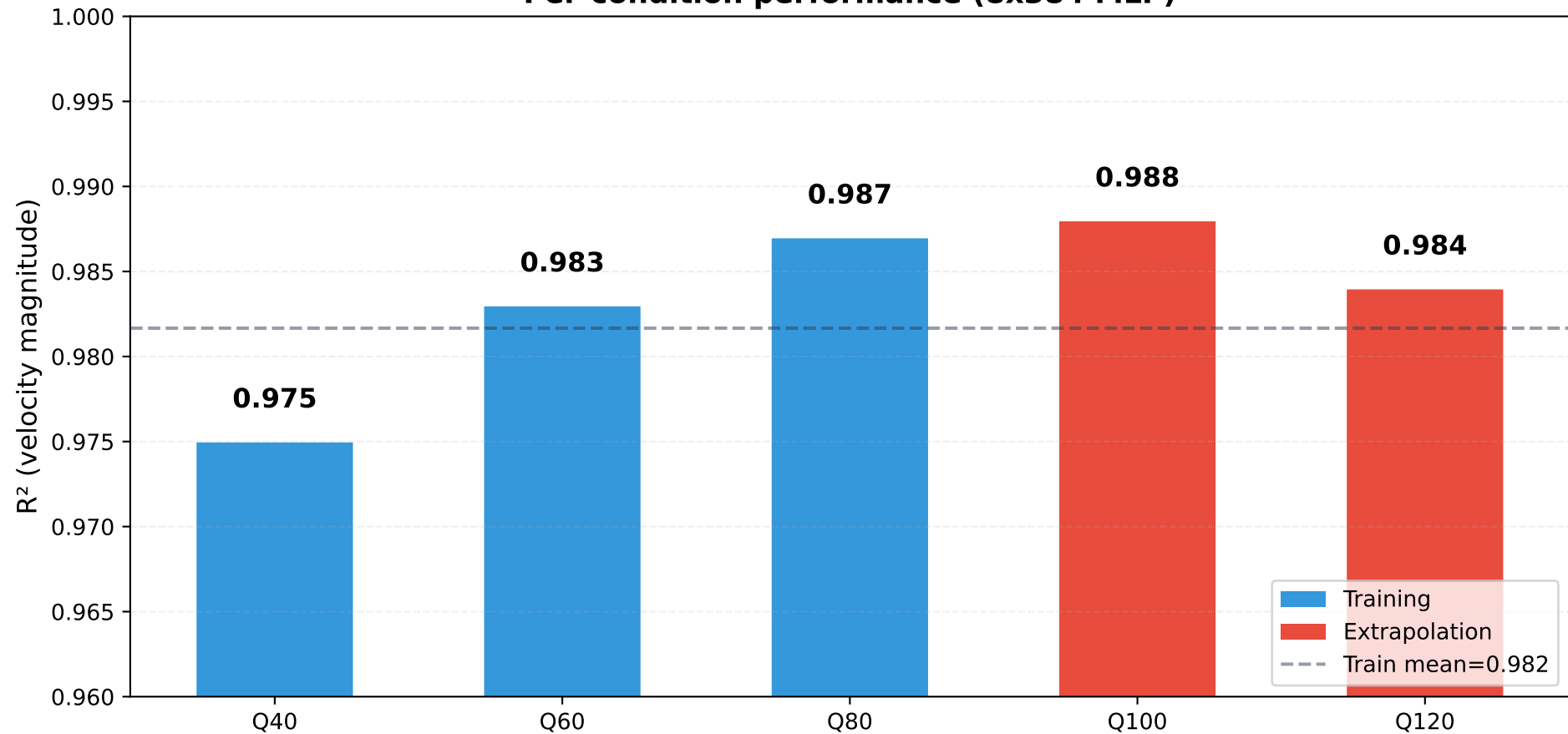
Per-condition performance (8x384 MLP)
