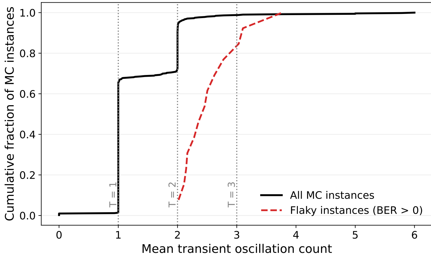
CDF of Transient Oscillation Metric
