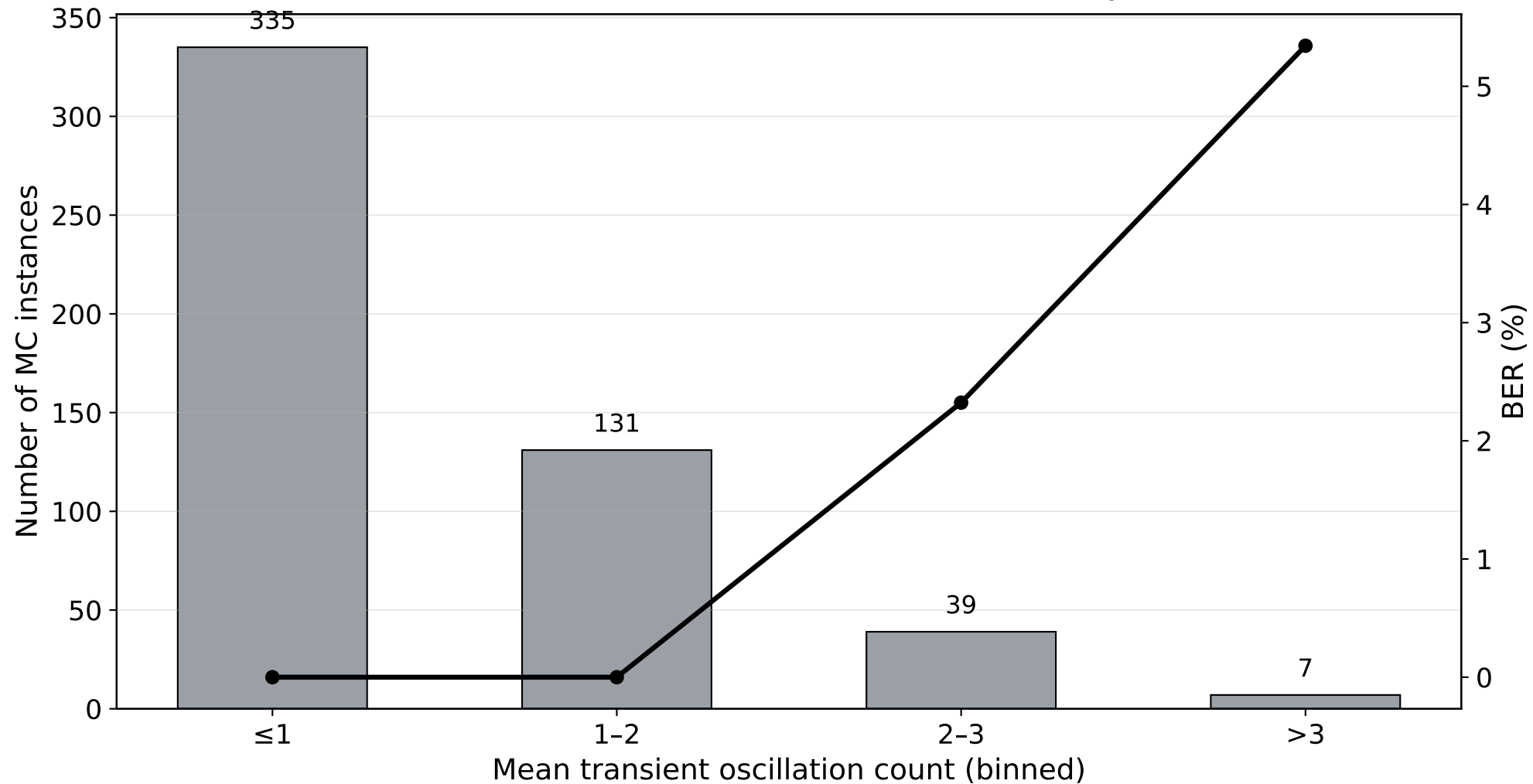
PUF BER vs. Transient Oscillation Activity
