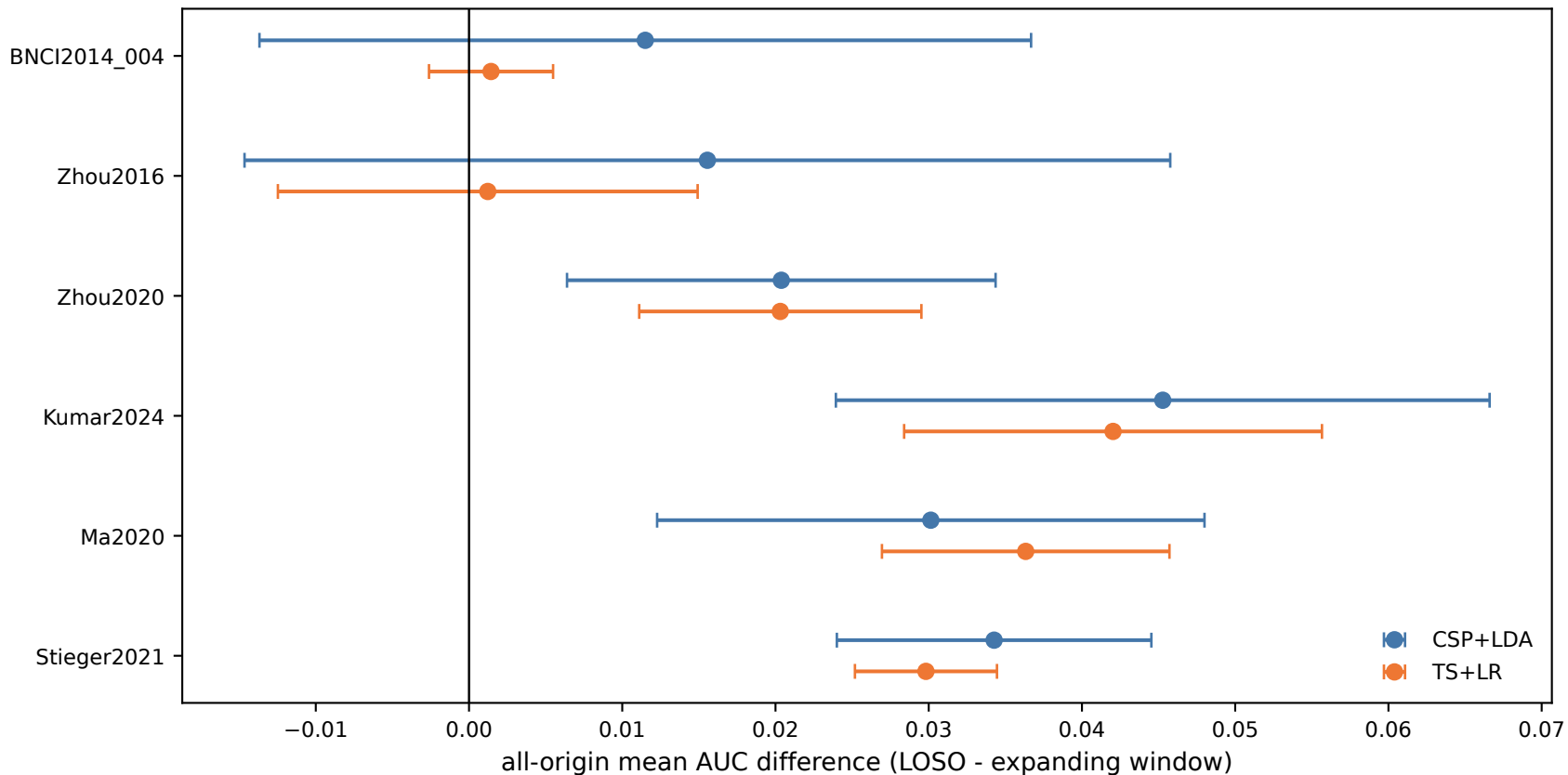
Primary protocol difference by dataset and decoder (95% CI)
