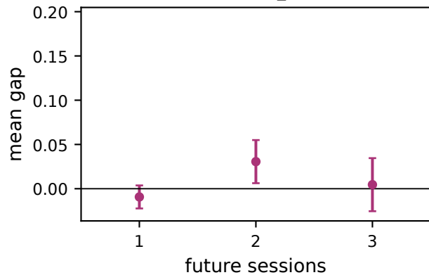
BNCI2014_004
