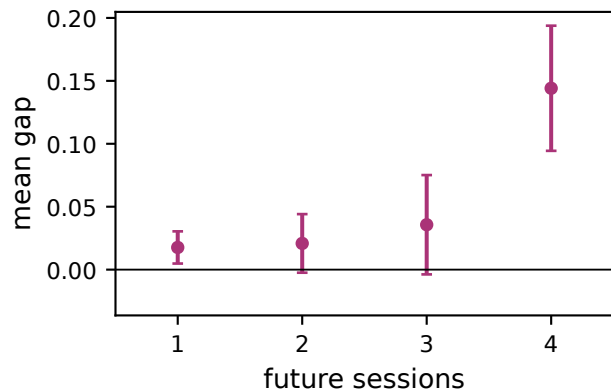
Kumar2024
