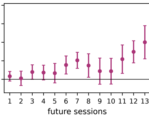
Ma2020
