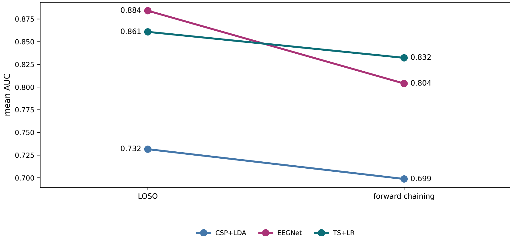
Model means under two evaluation protocols (Stieger2021, n=62) model order differs between protocols
