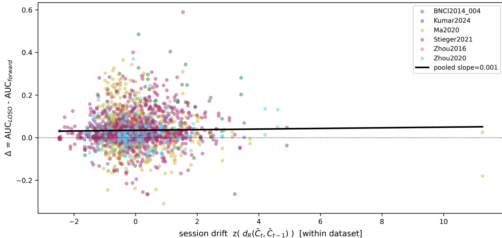
Protocol gap and consecutive-session covariance distance (raw observations and pooled descriptive line)
