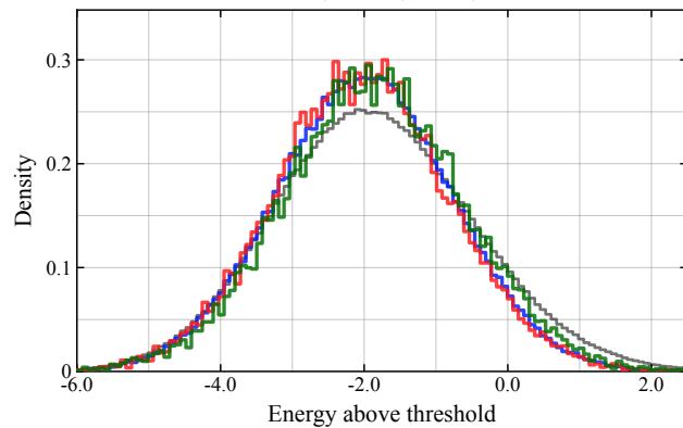
D. High-energy margin
