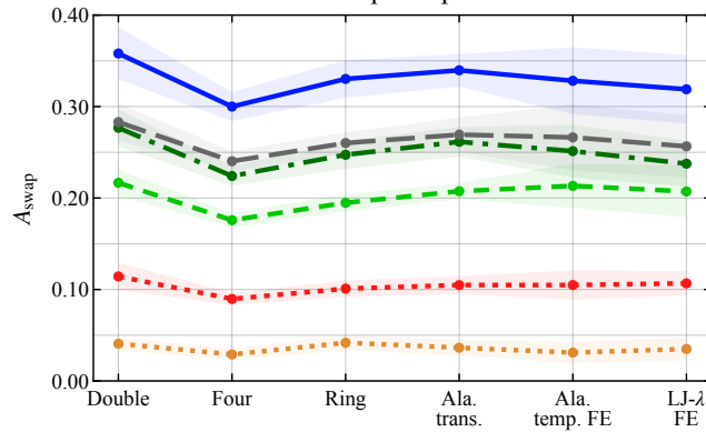
B. Swap acceptance
