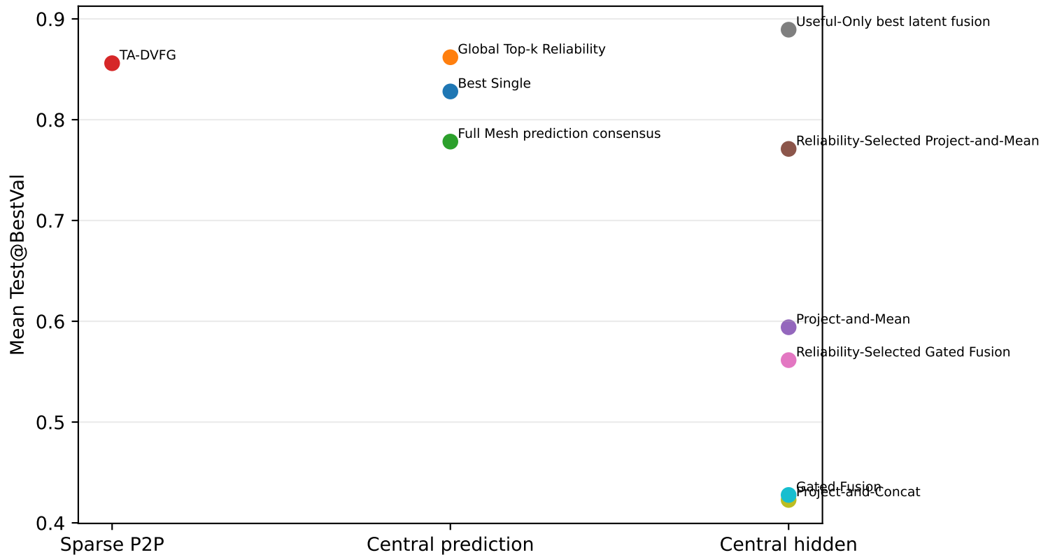
ACM Hard five-seed interface/performance trade-off
