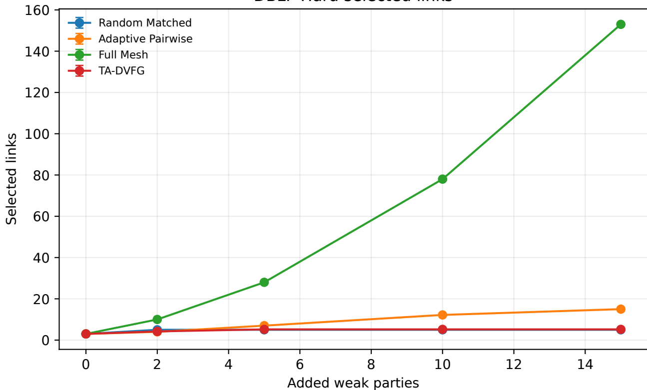
DBLP Hard selected links
