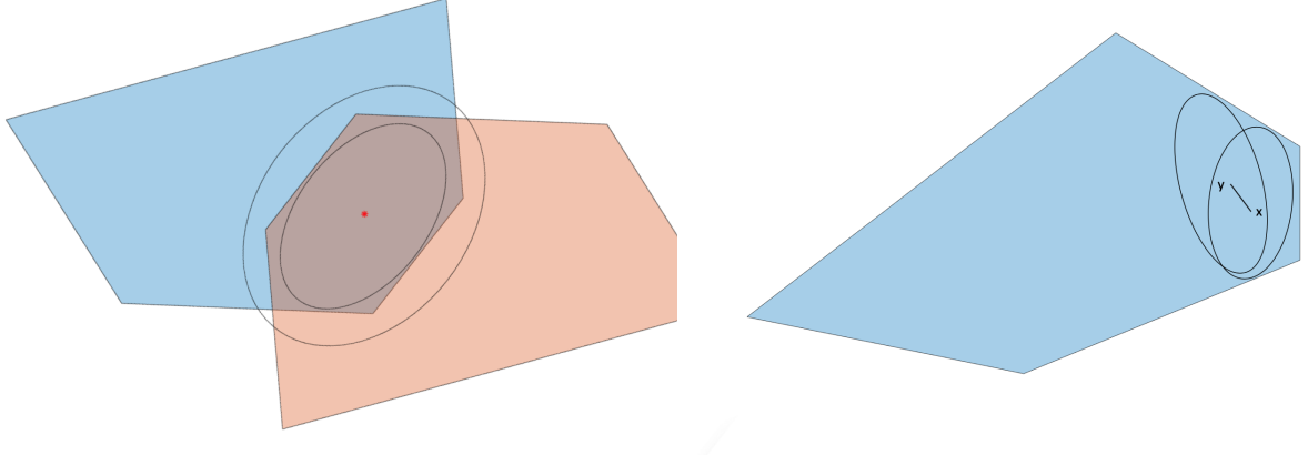
Figure 10.7: (a) E_u \subseteq K \cap (2u - K) \subseteq \alpha E_u . (b) Strong self-concordance measures the rate of change of Hessian of a barrier in the Frobenius norm
