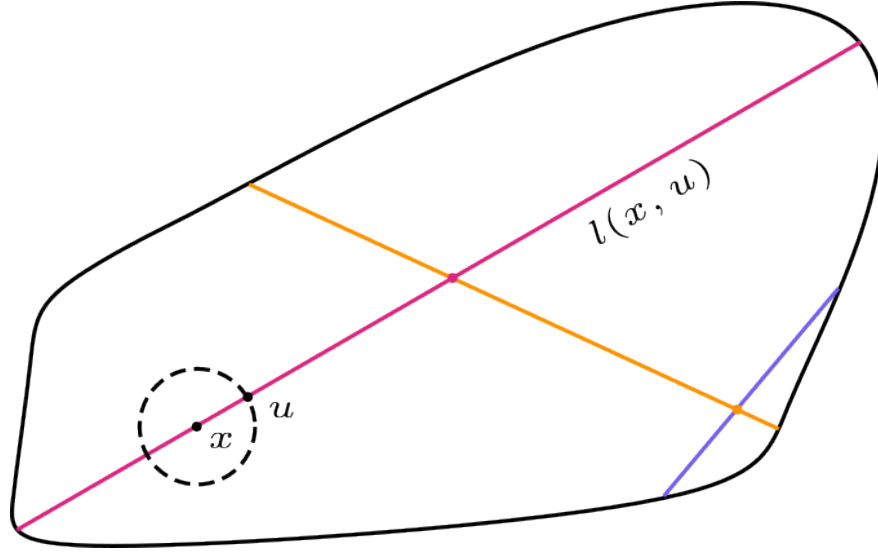
Figure 10.5: Hit-and-Run Algorithm
