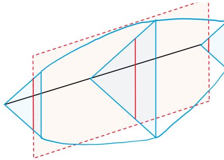
Figure 10.4: Going to an affine needle
