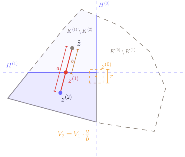
Figure 9.1: Algorithm (27) in its second iteration.
