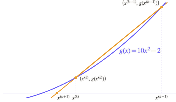
Figure 5.2: Secant Method
