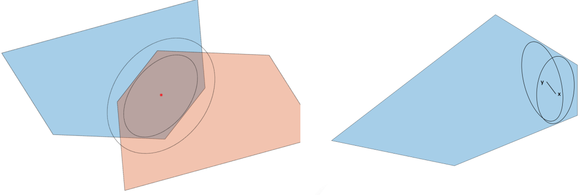
Figure 10.7: (a) E_u \subseteq K \cap (2u - K) \subseteq \alpha E_u . (b) Strong self-concordance measures the rate of change of Hessian of a barrier in the Frobenius norm
