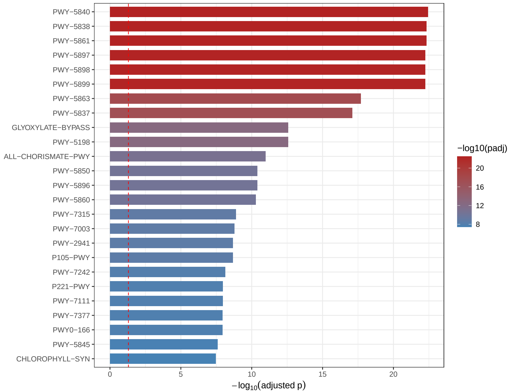
DESeq2 LRT: Top 25 Differential Pathways
