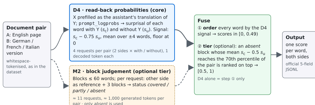
Figure 1. One document pair (English side A, other side B); both signals run in both directions. The solid path is the standalone system (D4); the dashed path adds the optional M2 tier.
