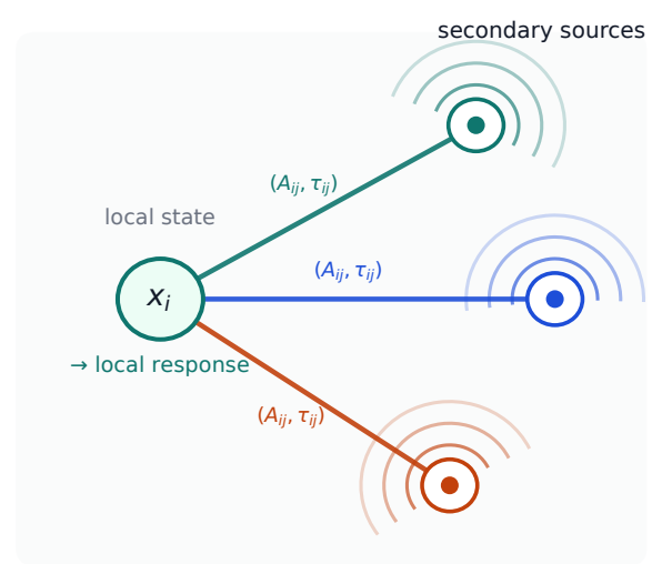
a Recursive local sources
