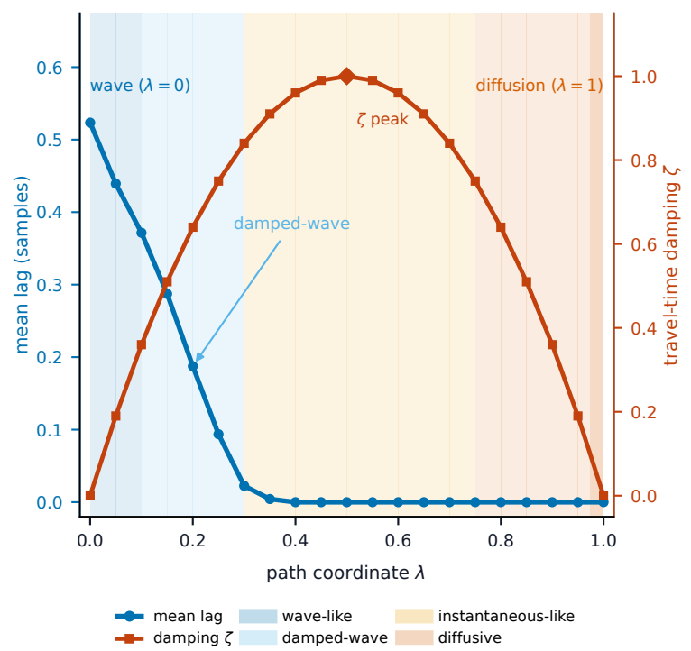
d Telegrapher path \Theta(\lambda) : wave → damped-wave → diffusion
