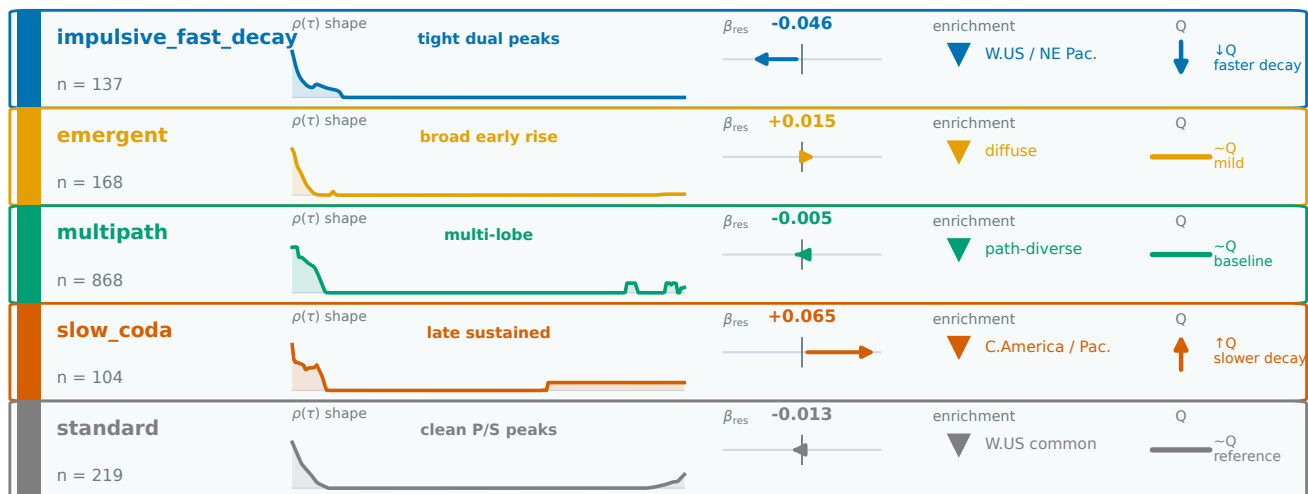
b Morphology-class characters ( \rho shape, \beta_{\text{res}} , enrichment, Q)
