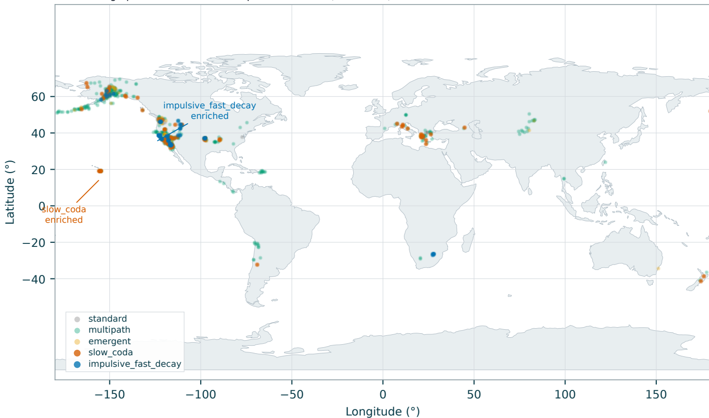
a Geographic enrichment of five operational facies (STEAD test)
