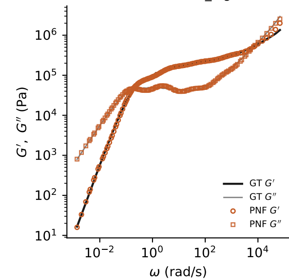
(c) PS1 T=170°C rel_log=0.030
