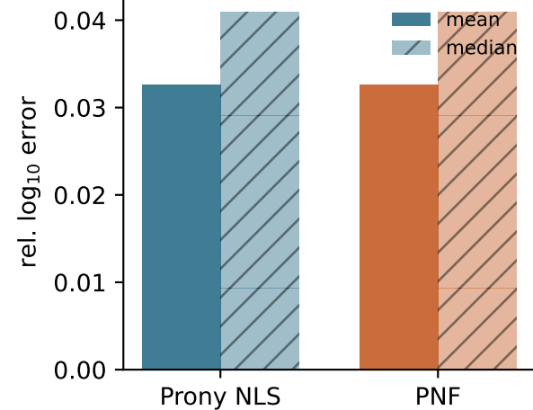
(a) Fixed- \lambda library fit
