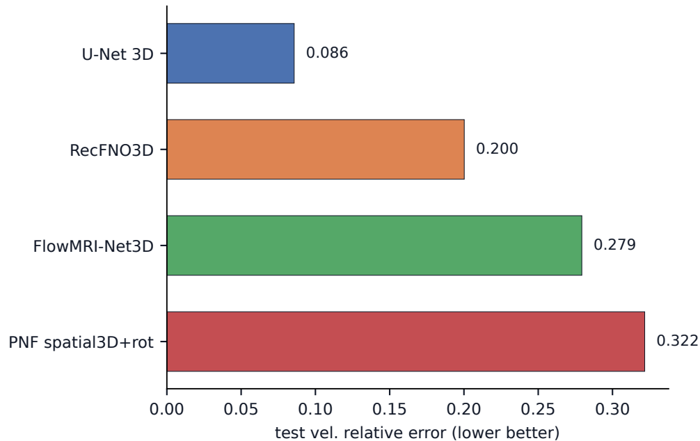
vortex_tube @10% keep
