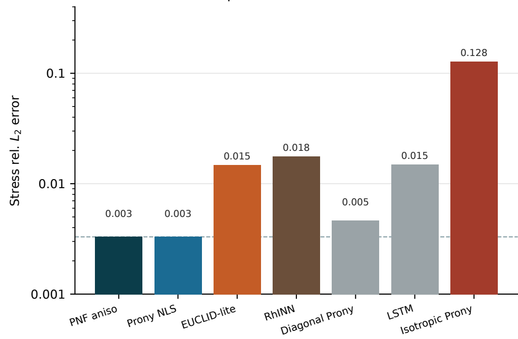
a Model zoo — stress prediction error
