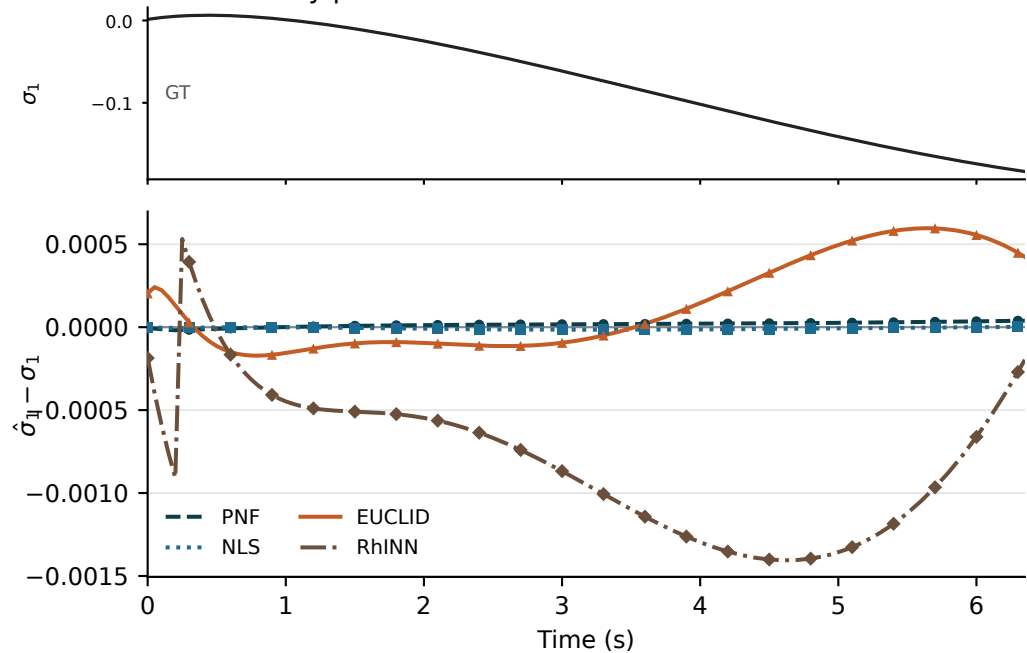
d Oscillatory protocol — GT stress & residual
