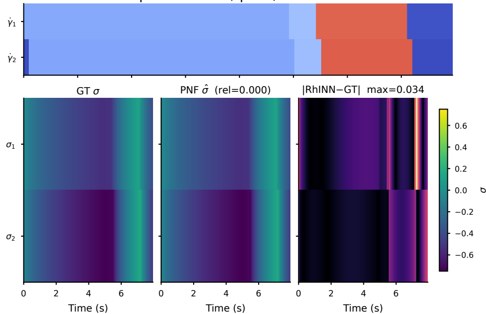
c Case: multi-step shear — GT / pred / error
