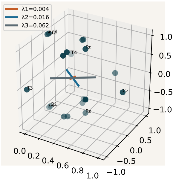
Learned anisotropy D on 10-20
