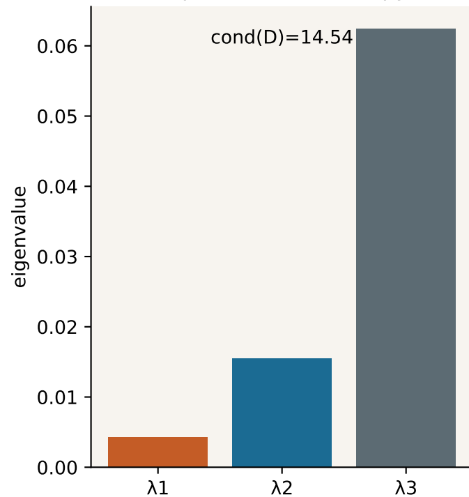
D spectrum (anisotropy)
