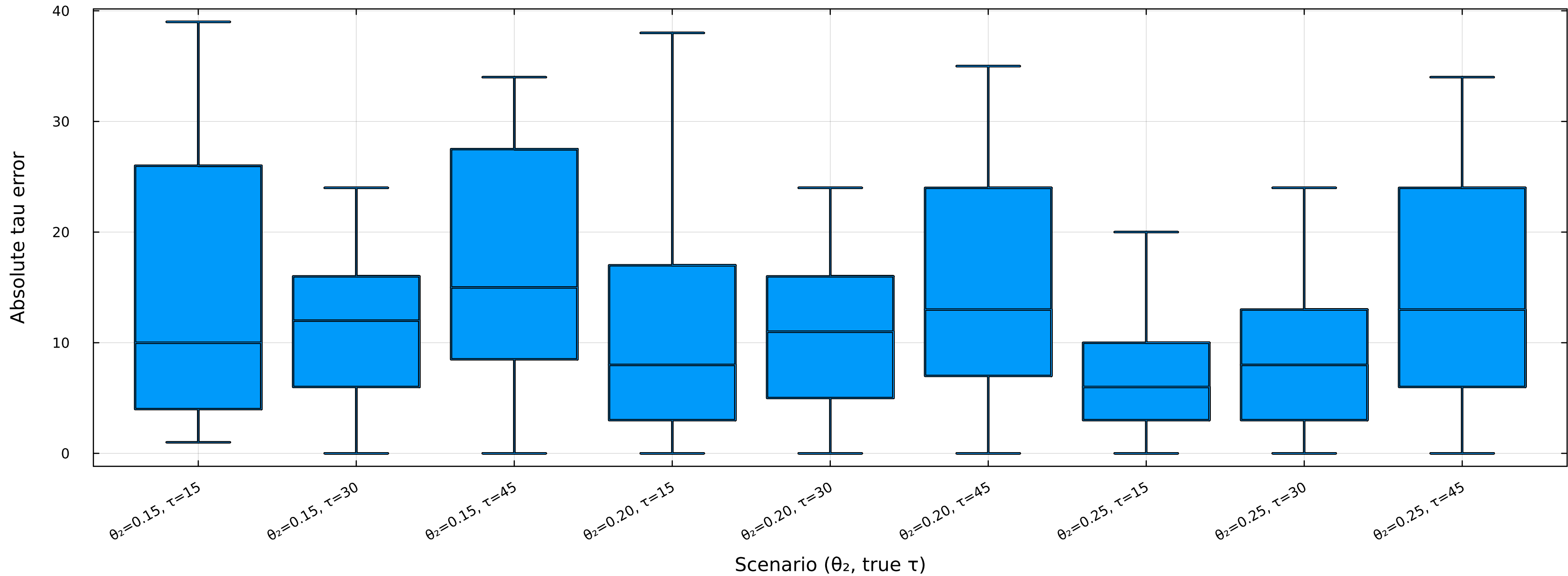
Changepoint localization error
