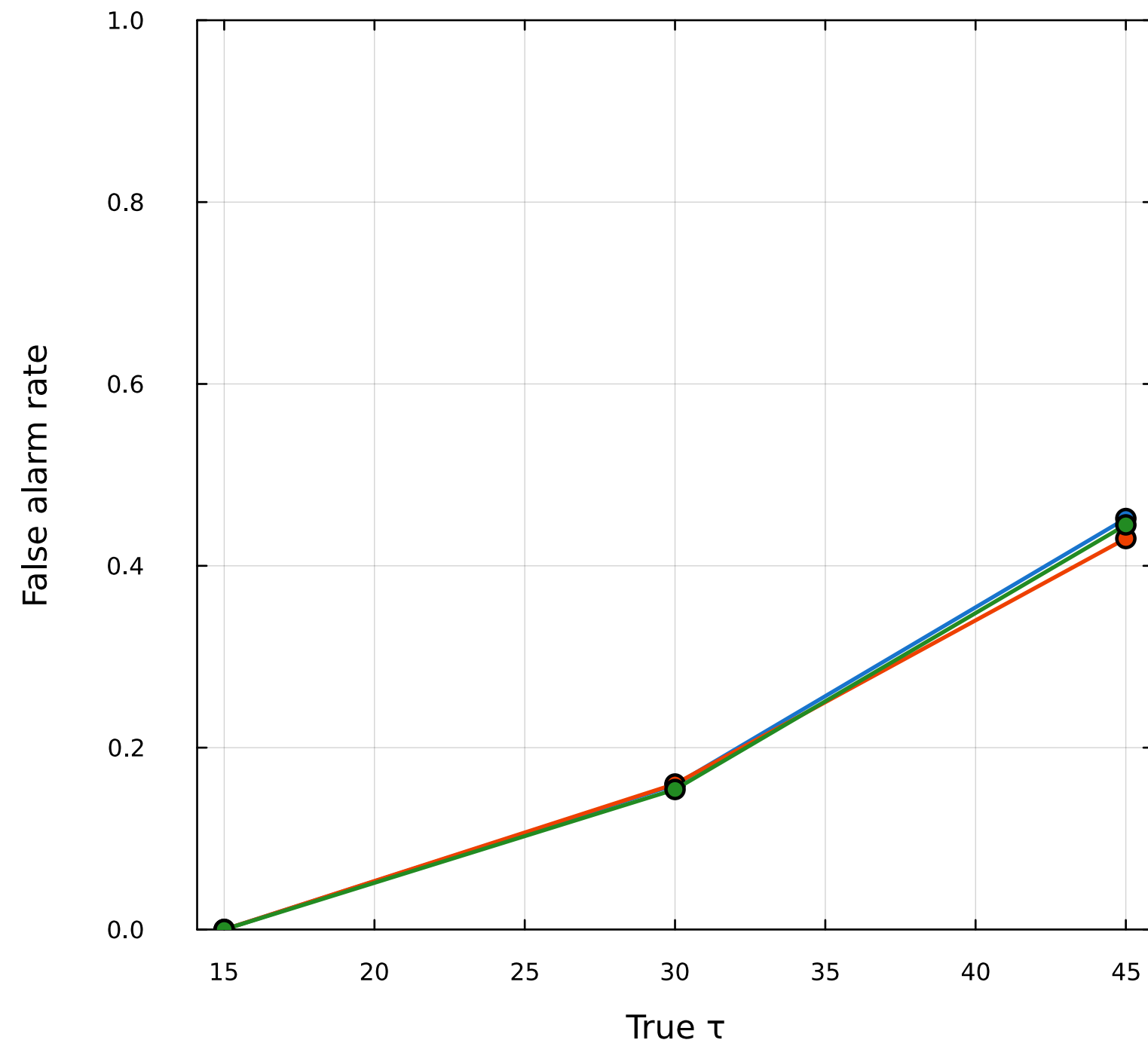
False alarms
