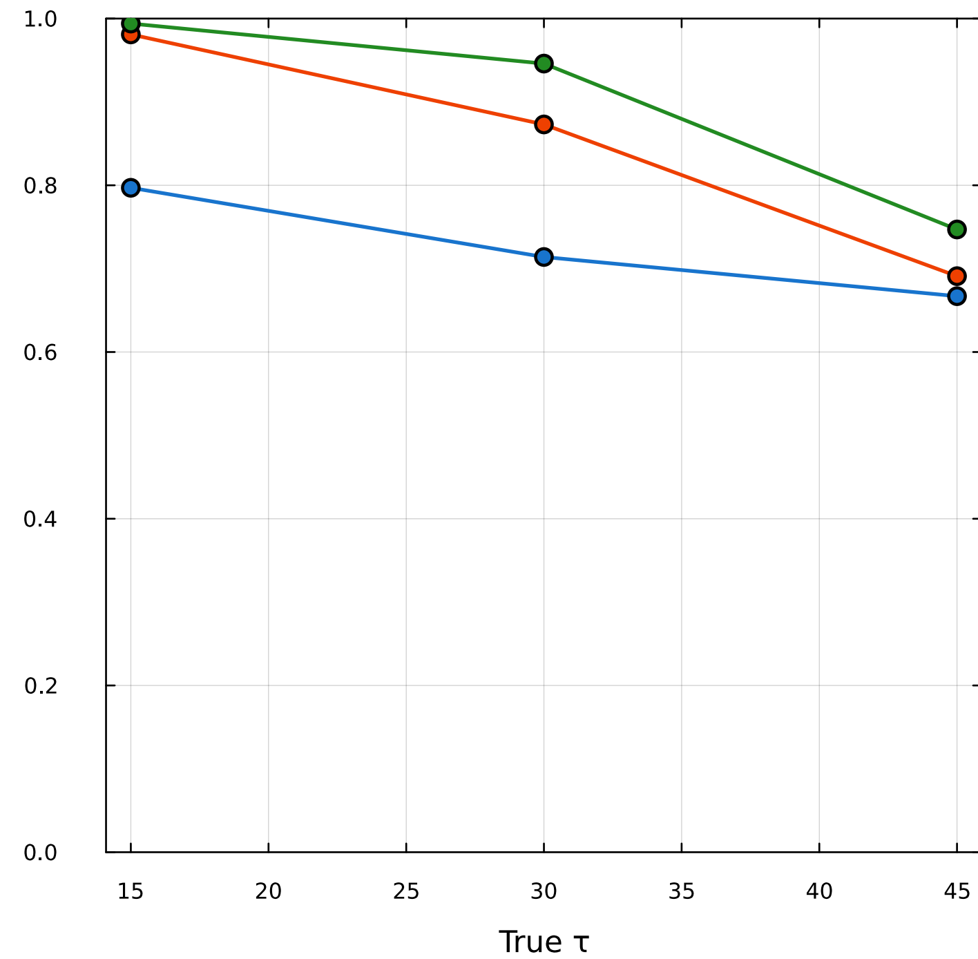
Detection
