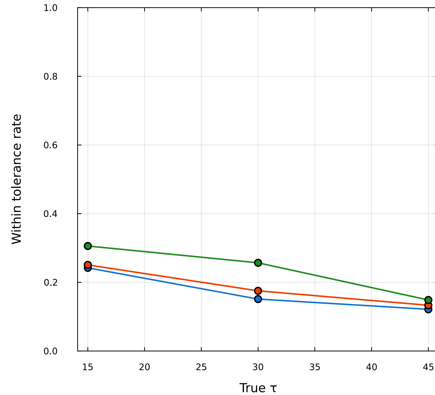
Tau accuracy
