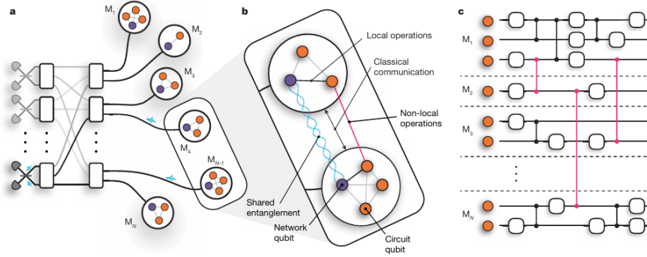
FIG. 9: (a) conceptual diagram of the QGT with multiple modules, (b) QGT setup, (c) physical connection between multiple modules. By Main et al. [11].
