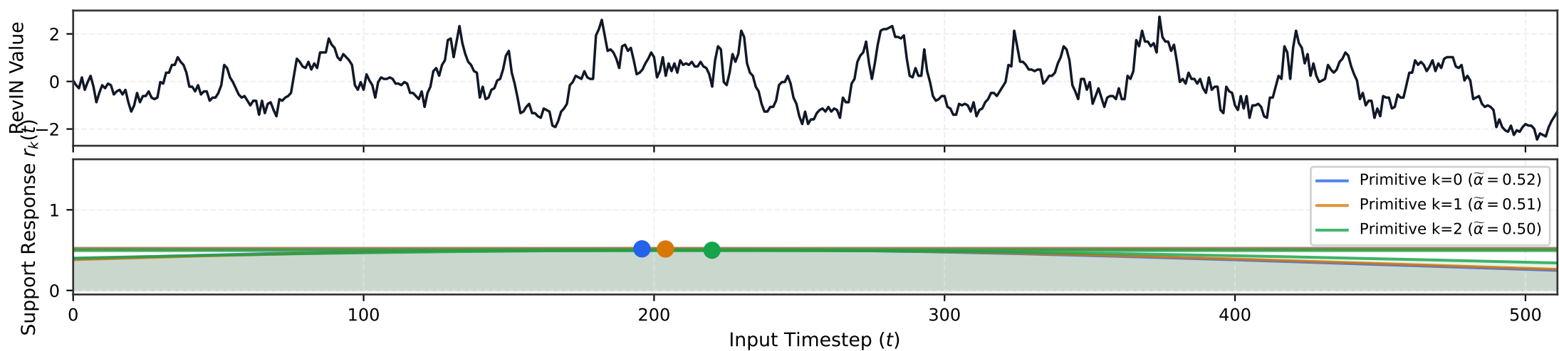
ETTm1 (High Complexity, \kappa = 13.70 ) | Active Primitives K(x) = 3
