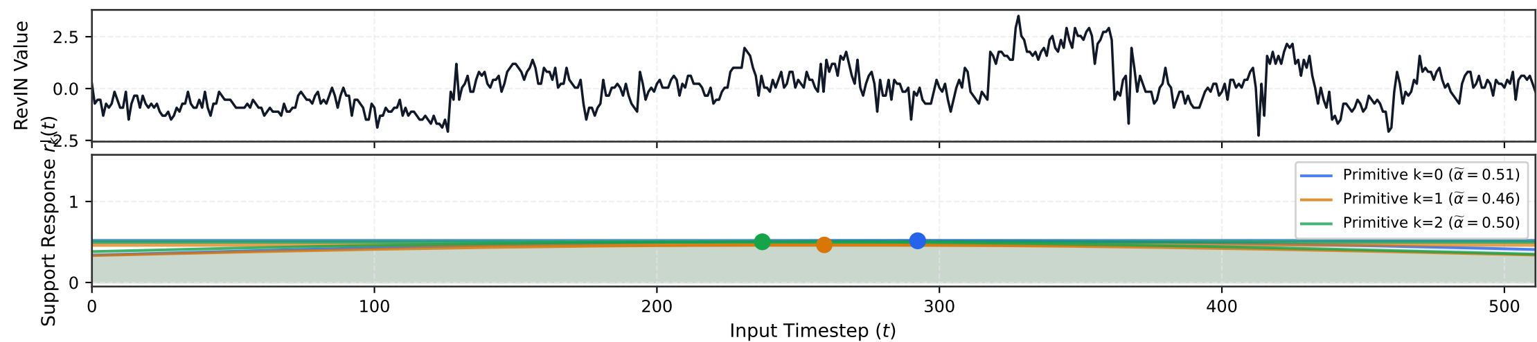
ETTm1 (High Complexity, \kappa = 13.70 ) | Active Primitives K(x) = 3
