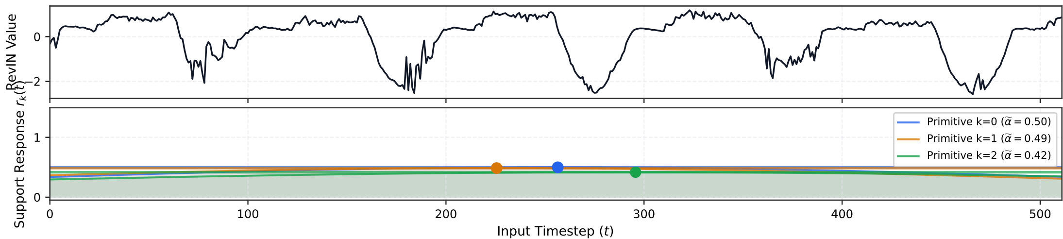
ETTm1 (Medium Complexity, \kappa = 9.65 ) | Active Primitives K(x) = 3
