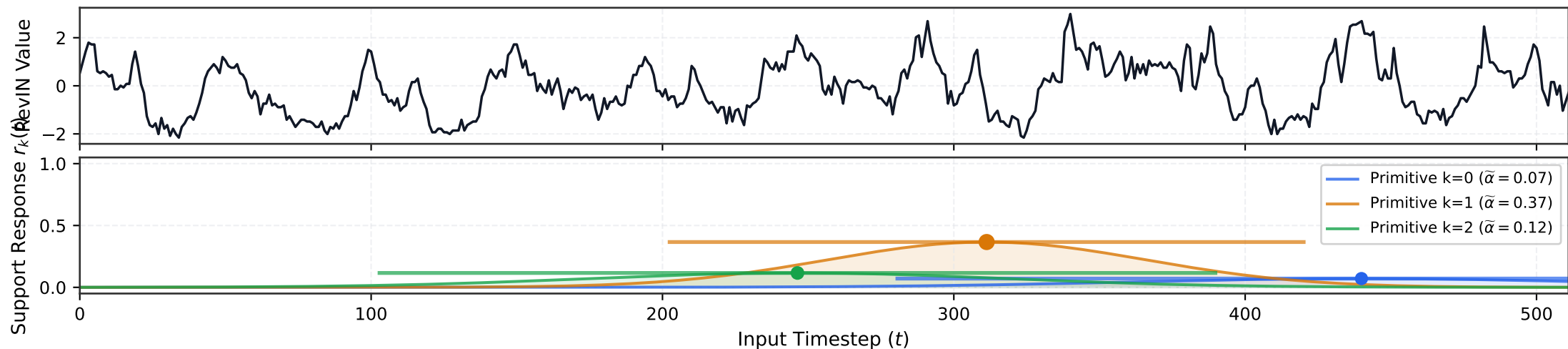
ETTm1 (High Complexity, \kappa = 14.06 ) | Active Primitives K(x) = 3
