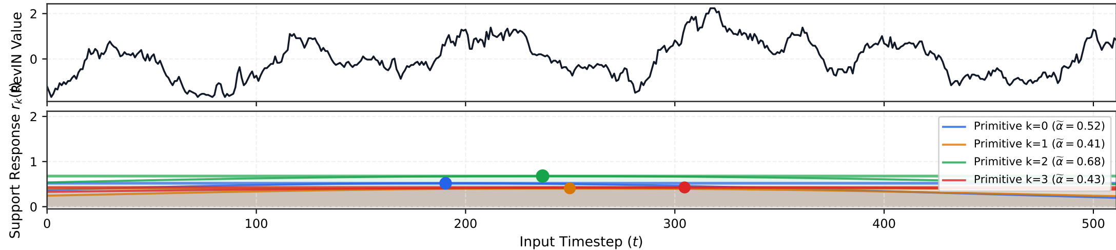
ETTm1 (Medium Complexity, \kappa = 10.23 ) | Active Primitives K(x) = 3
