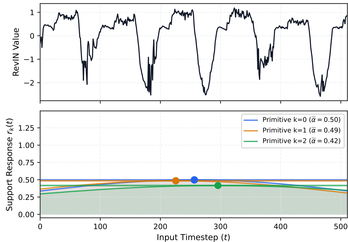
ETTm1 (Low Complexity, \kappa = 4.90 ) | Active Primitives K(x) = 3
