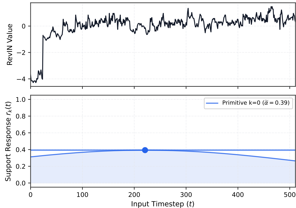
ETTh1 (Low Complexity, \kappa = 5.42 ) | Active Primitives K(x) = 1
