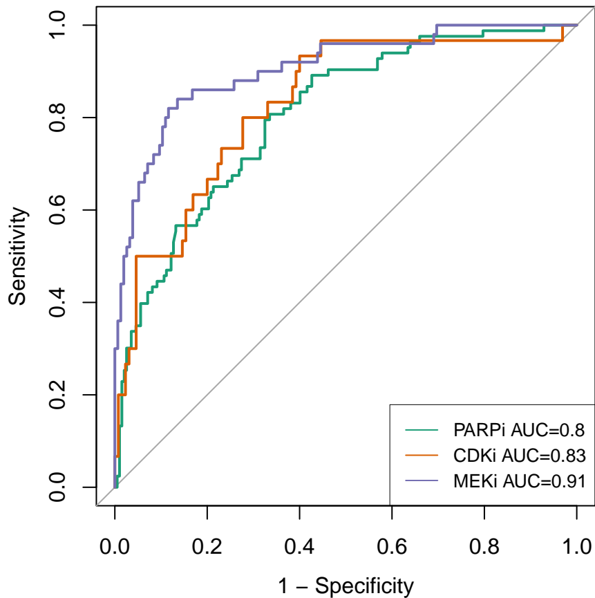
ROC of validate datasets
